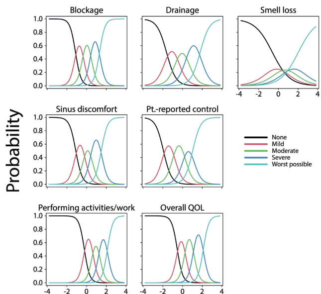
Figure 6. Item characteristic curves for items of the CRCT sinonasal (top two rows) and impairment (bottom row) subdomains.
