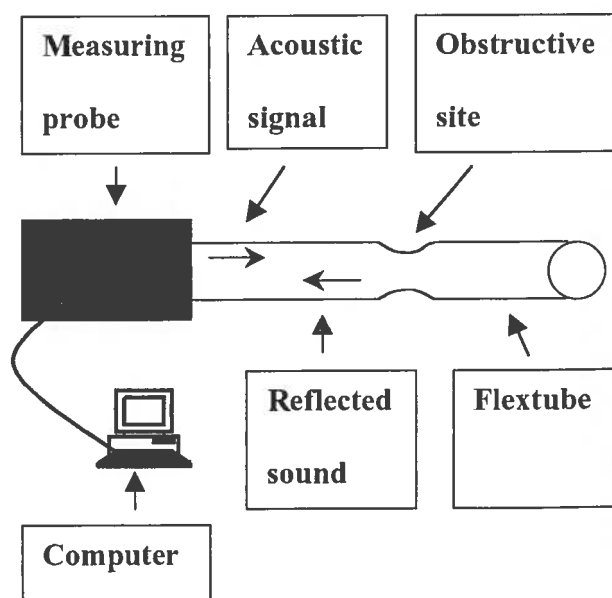
Figure 1. The flextube reflectometry system. A continuous white band noise was generated in the probe and sent into the flextube. The flextube was inserted into the nose, pharynx and oesophagus. When the flextube was narrowed during obstructions the noise was reflected. A microphone in the probe recorded the reflected sound. The distance to the obstructive site and the duration of obstructions was calculated by the measuring system and graphically illustrated by the software
