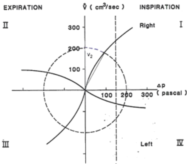
Figure 1. Broms' model for active anterior rhinomanometry: v_2 is the angle between the flow axis and a line through the origin to the point where the \Delta p/V -curve intersects a circle with a radius of 200 (200 Pascal or 200 \text{cm}^3/\text{s} ). This expresses the nasal airway resistance NAR ( R_2 = \tan v_2 ), i.e. v_2 = 20^\circ correspond to R_2 = 0.36 \text{ Pa}/(\text{cm}^3/\text{s}) and R_{150} = 0.48 \text{ Pa}/(\text{cm}^3/\text{s}) . Another approach according to the committee report on standardization of rhinomanometry is to express the resistance at a fixed pressure of 150 Pascal, R_{150} .
