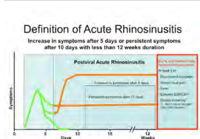
Figure 2.2 Definition of ARS
