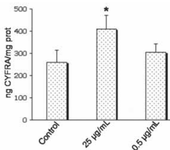
Figure 4. Cytokeratin 19 expressed as ng of CYFRA per mg of intracellular protein content (*) refers to a significant difference from the control ( p < 0.01 ).
